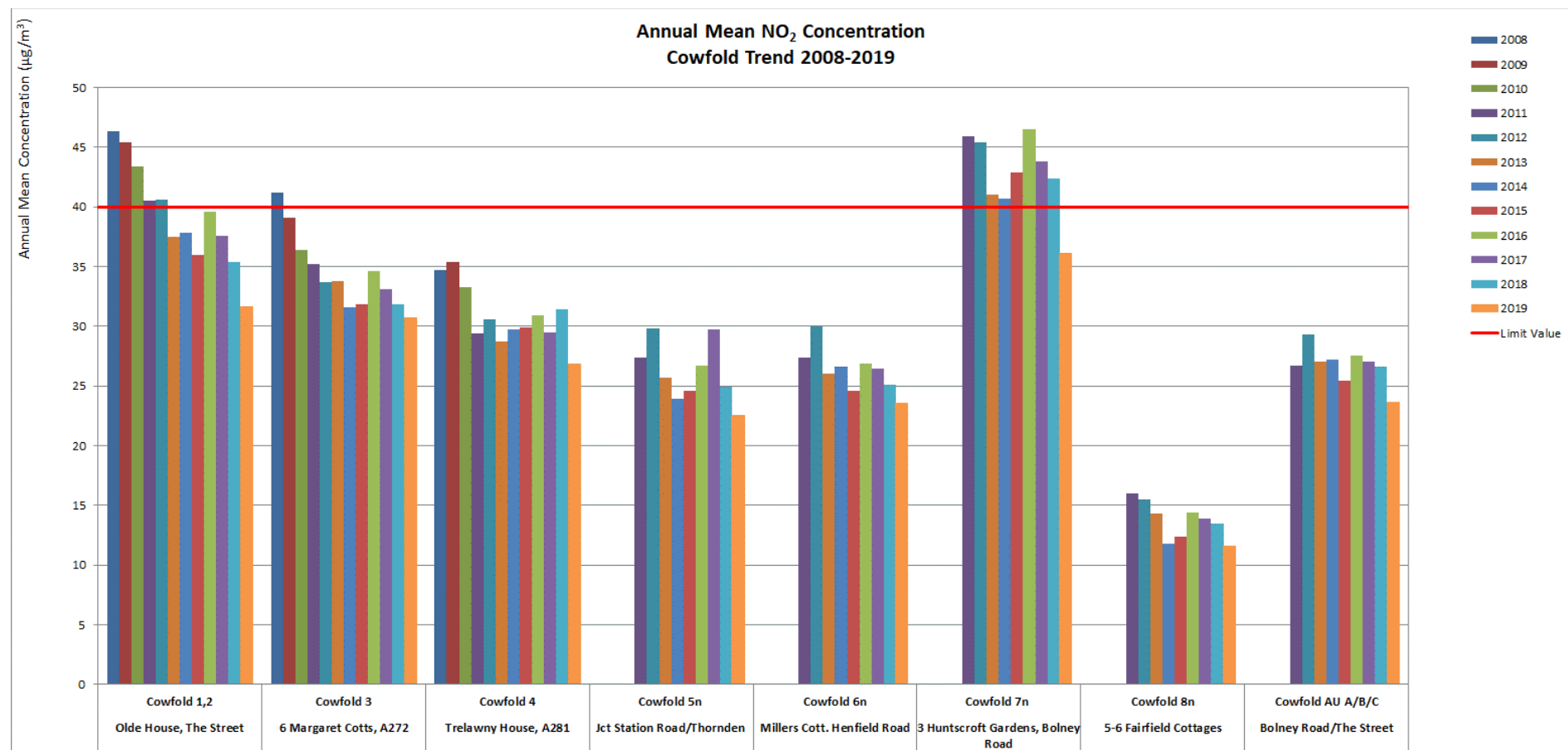
Figure A6 – Trends in Annual Mean NO 2 Concentrations measured at Diffusion Tube Monitoring Sites 2008 – 2019: Cowfold
