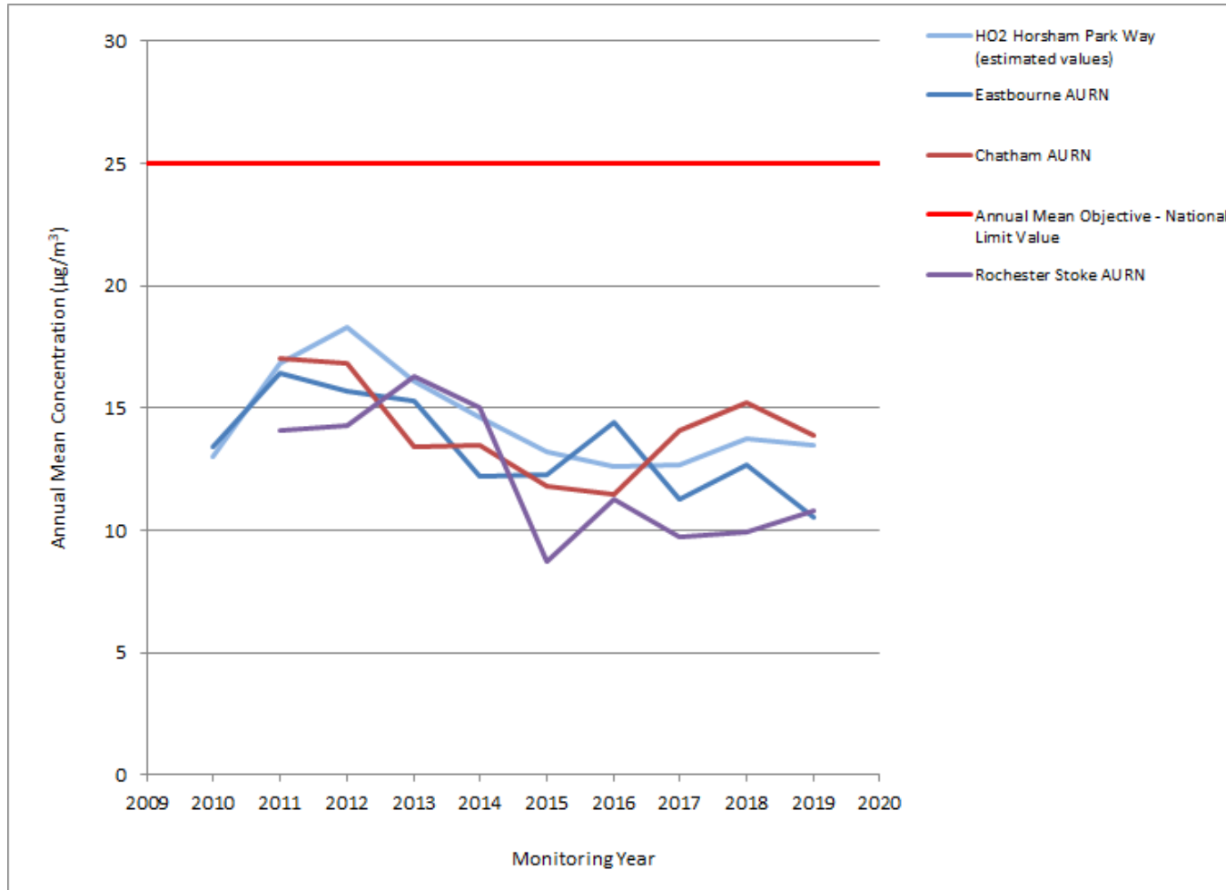
Figure A3 – Trends in Annual Mean PM 2.5 Concentrations Measured at Automatic Monitoring Sites 2010 – 2019
