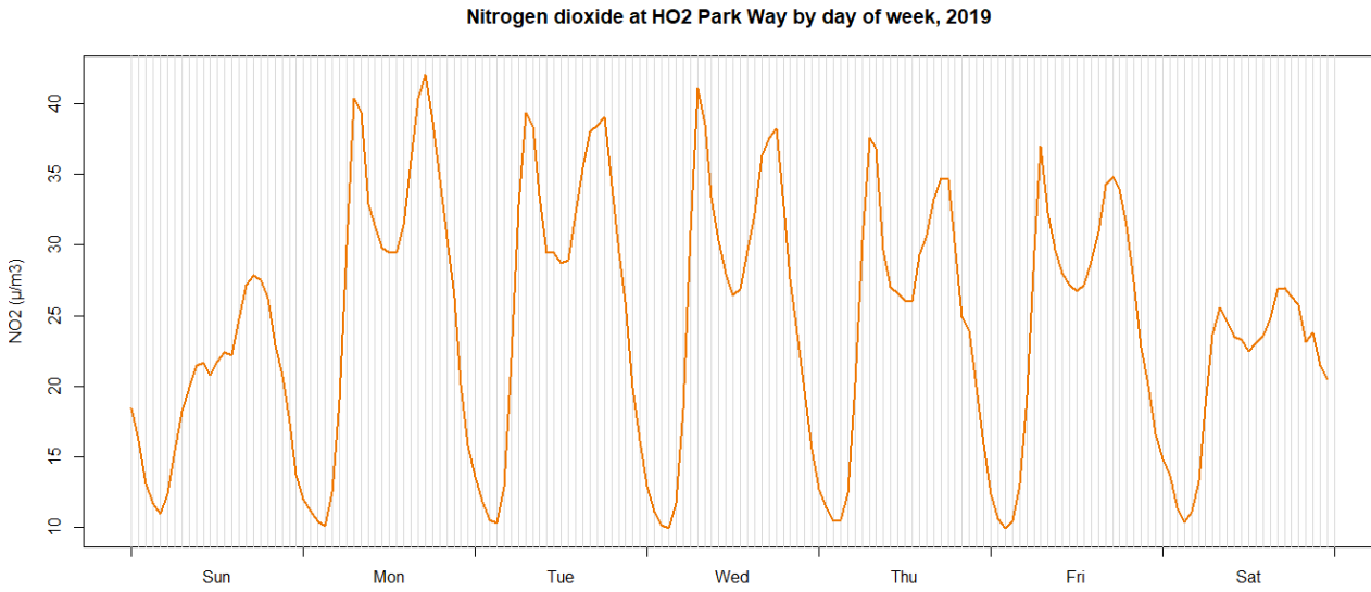
Figure B7 – Continuous Monitoring Results: Day of Week Concentrations for NO 2 at HO2 Horsham Park Way, 2019
