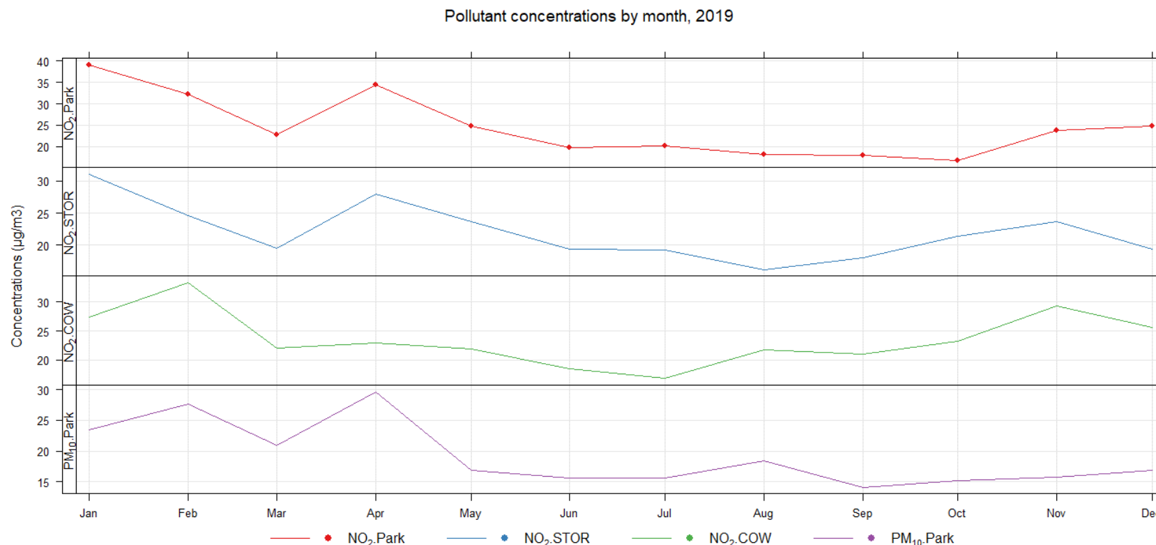
Figure B3 – Continuous Monitoring Results: Monthly Concentrations for NO 2 and PM 10 at HO2 Horsham Park Way, HO4 Storrington AURN & HO5 Cowfold in 2019
