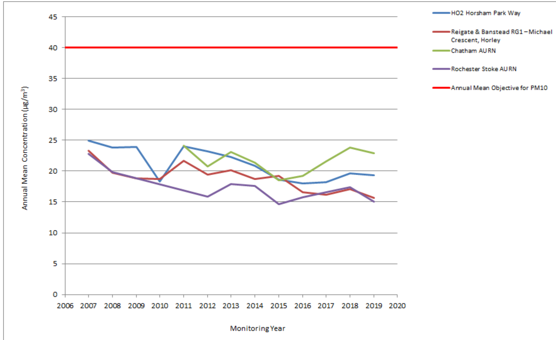
Figure A2 – Trends in Annual Mean PM 10 Concentrations Measured at Automatic Monitoring Sites 2007 – 2019
