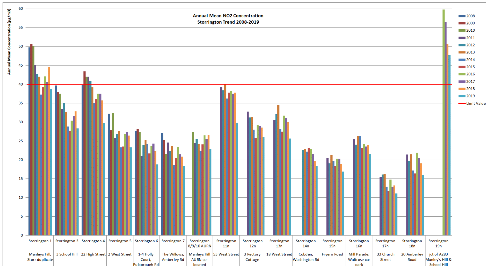
Figure A5 – Trends in Annual Mean NO 2 Concentrations measured at Diffusion Tube Monitoring Sites 2008 – 2019: Storrington
