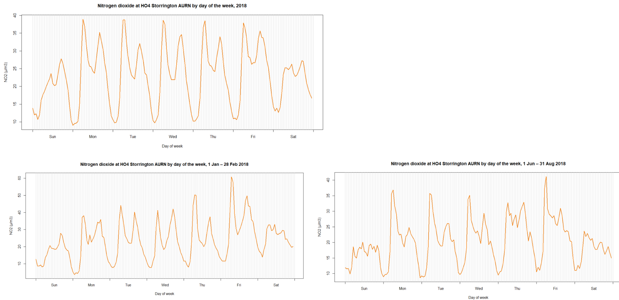
Figure B9 – Continuous Monitoring Results: Day of Week Concentrations for NO 2 at HO4 Storrington AURN, 2018
