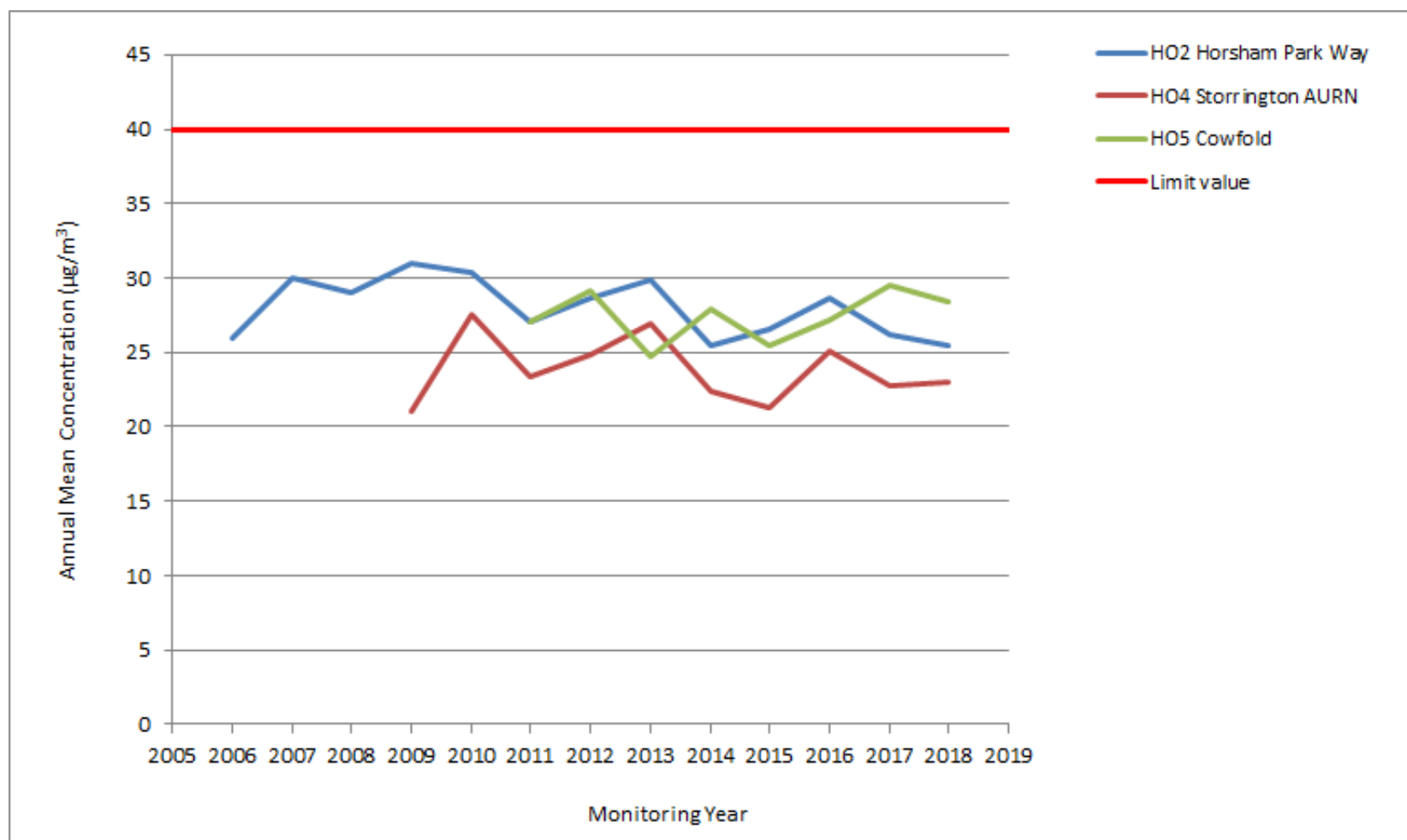
Figure A1 – Trends in Annual Mean NO 2 Concentrations Measured at Automatic Monitoring Sites 2006 – 2018
