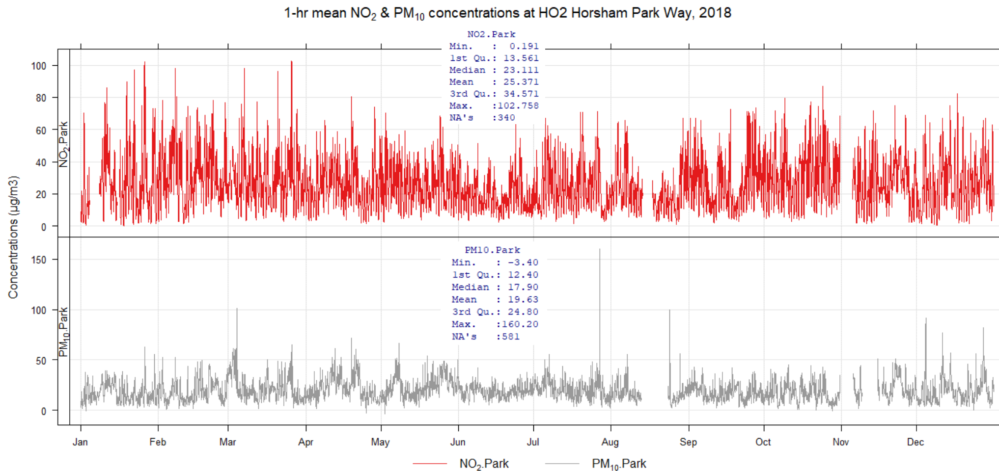
Figure B1 – Continuous Monitoring Results: 1-hr mean NO 2 & PM 10 Concentrations, HO2 Horsham Park Way, 2018
