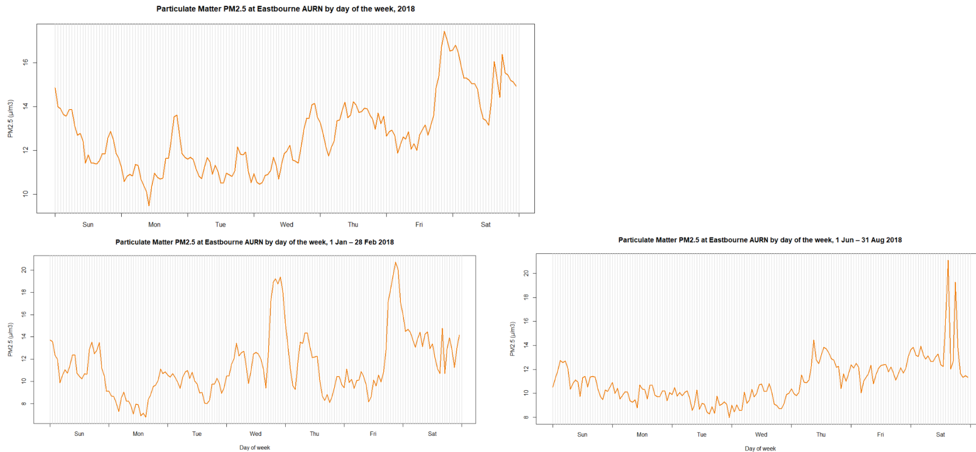
Figure B15 – Continuous Monitoring Results: Day of Week Concentrations for PM 2.5 at Eastbourne, 2018
