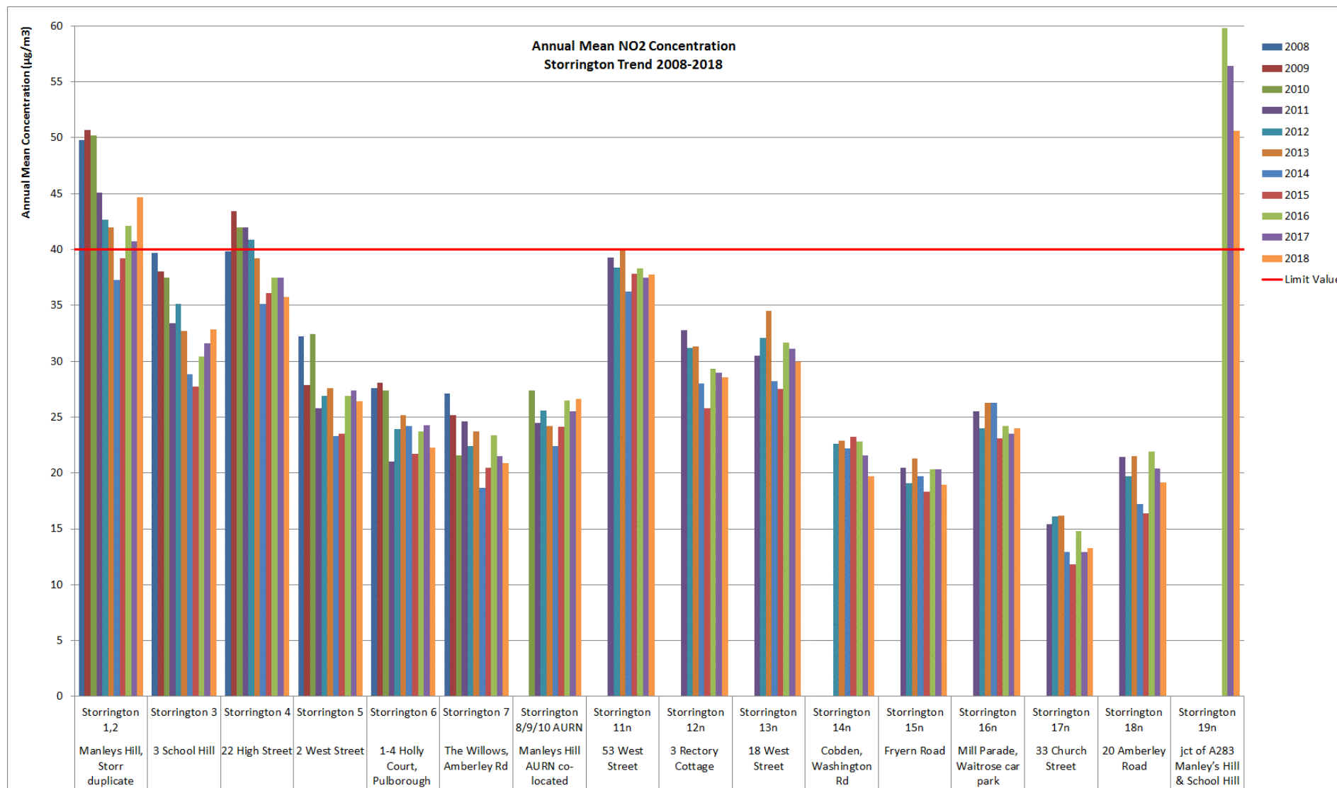
Figure A5 – Trends in Annual Mean NO 2 Concentrations measured at Diffusion Tube Monitoring Sites 2008 – 2018: Storrington
