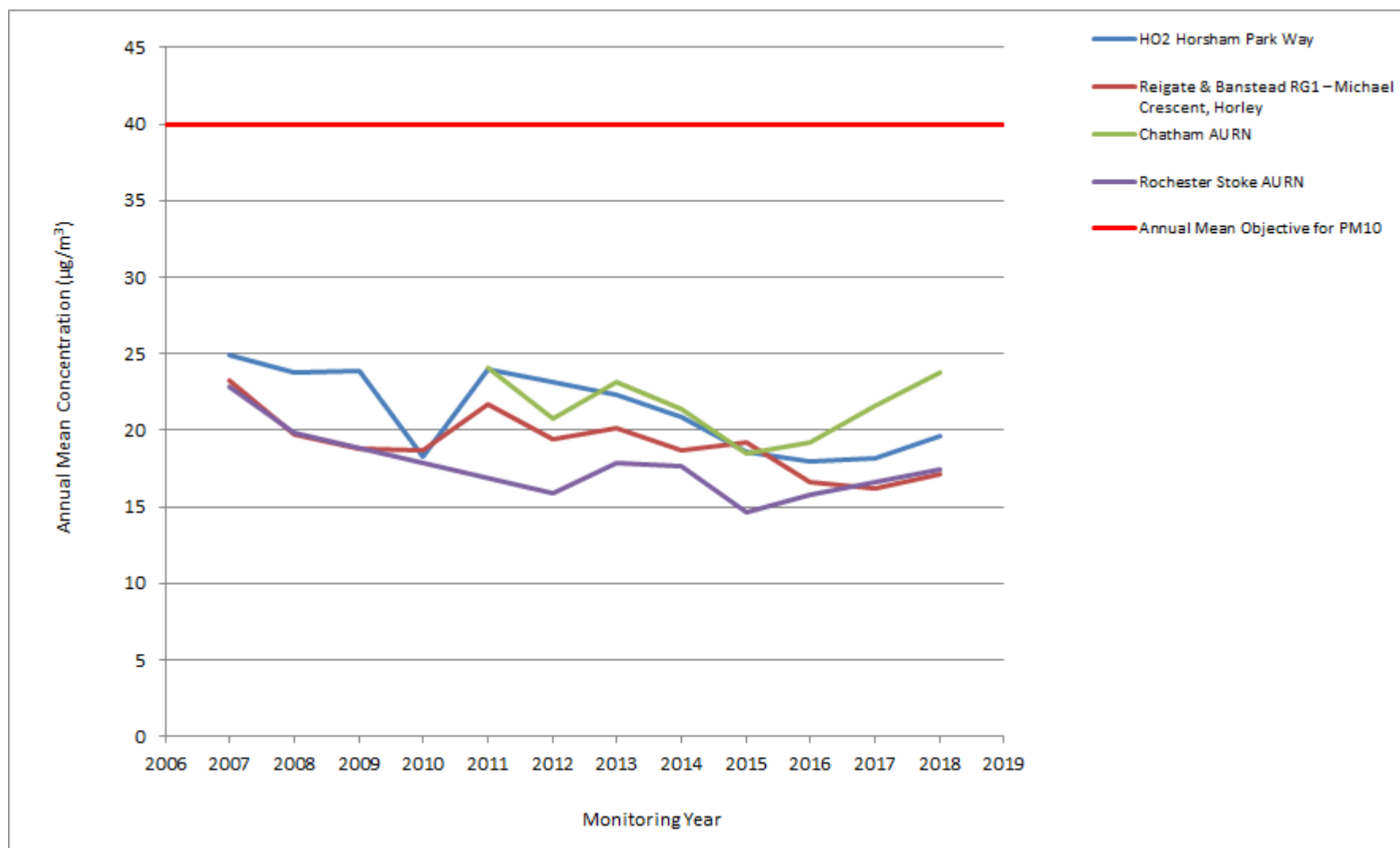
Figure A2 – Trends in Annual Mean PM 10 Concentrations Measured at Automatic Monitoring Sites 2007 – 2018
