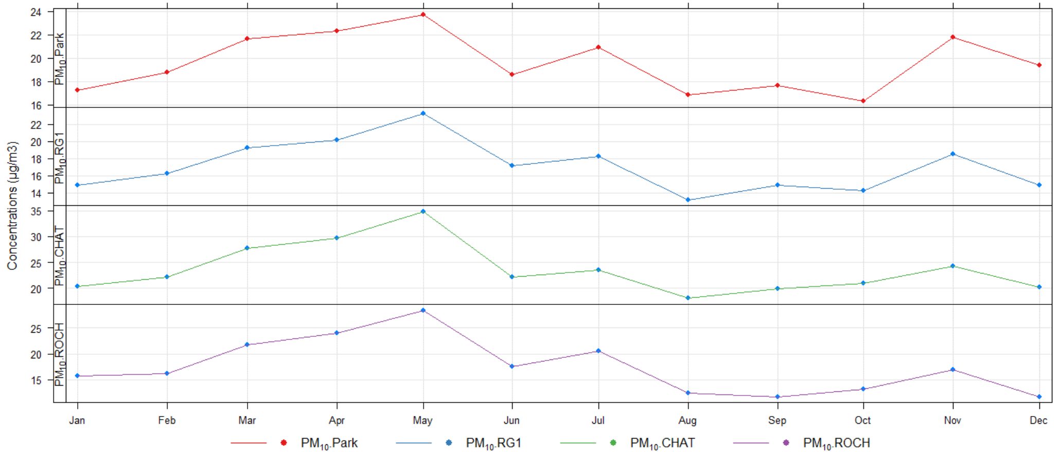
PM 10 concentrations by month, 2018
