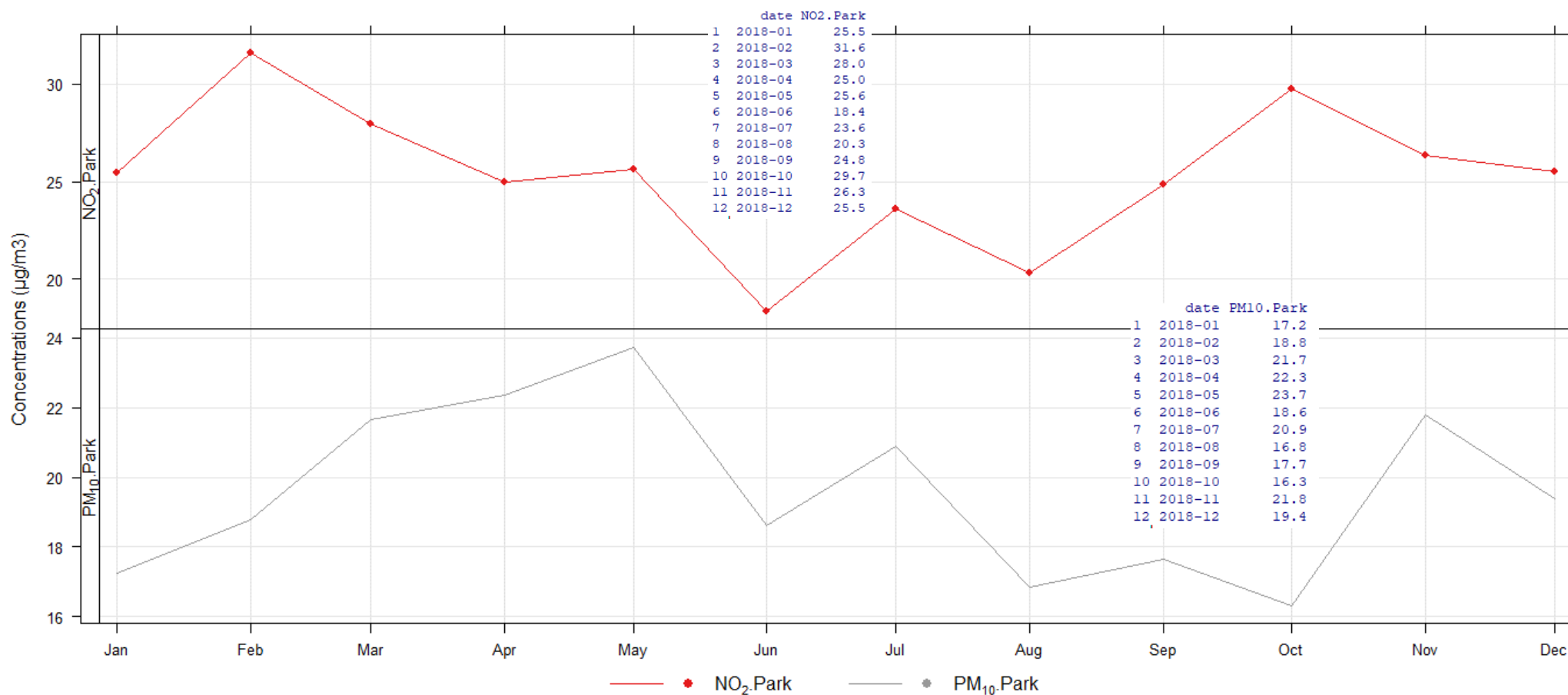
Pollutant concentrations by month, 2018
