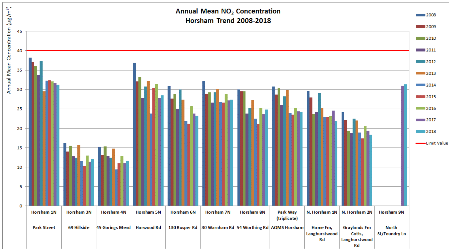
Figure A4 – Trends in Annual Mean NO 2 Concentrations measured at Diffusion Tube Monitoring Sites 2008 – 2018: Horsham
