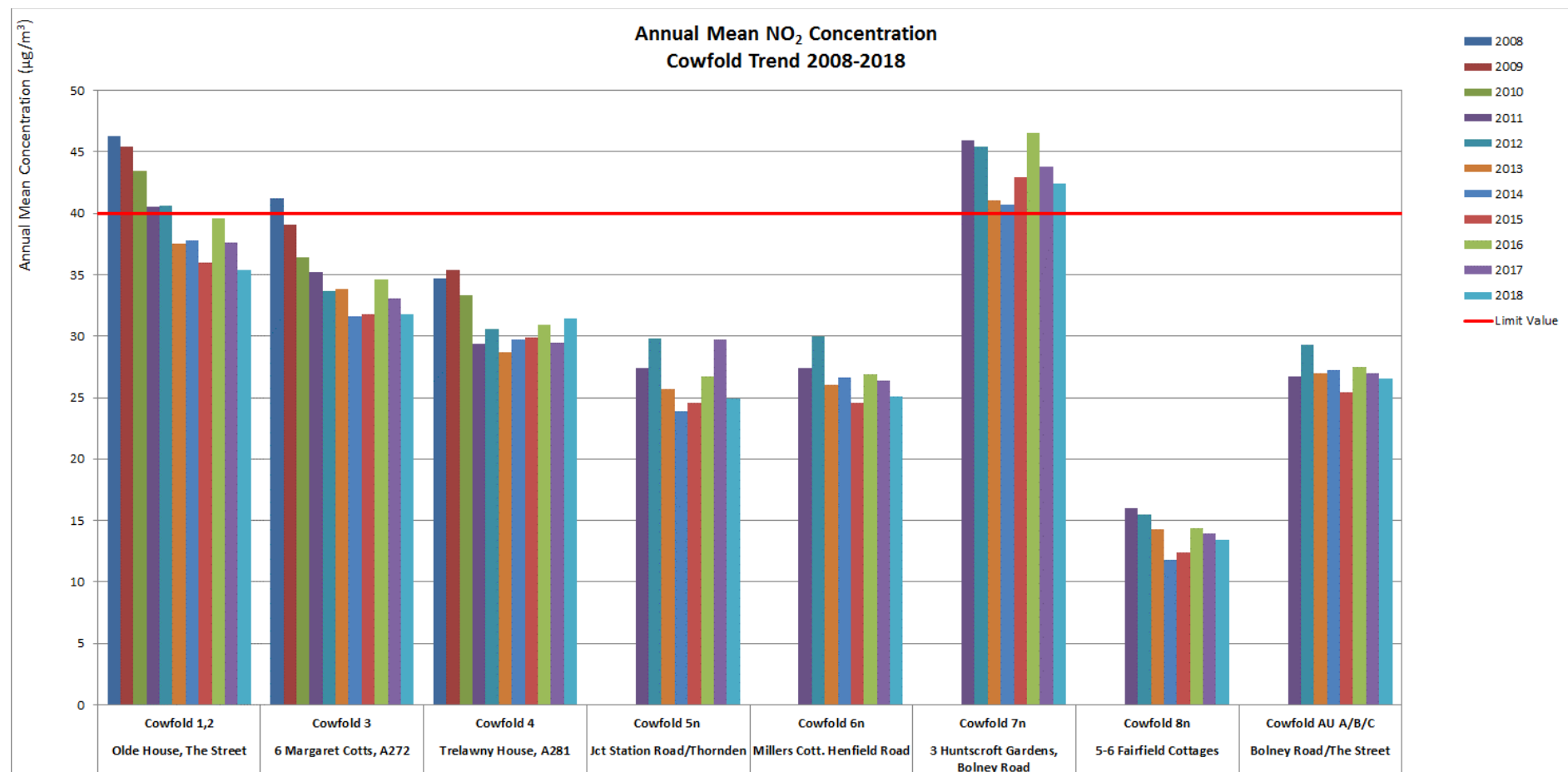
Figure A6 – Trends in Annual Mean NO 2 Concentrations measured at Diffusion Tube Monitoring Sites 2008 – 2018: Cowfold
